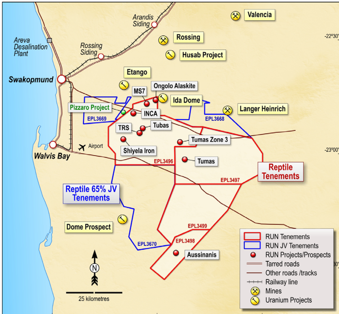
Figure 1: Location map for the Nova Energy and Reptile Uranium Namibia EPLs.
