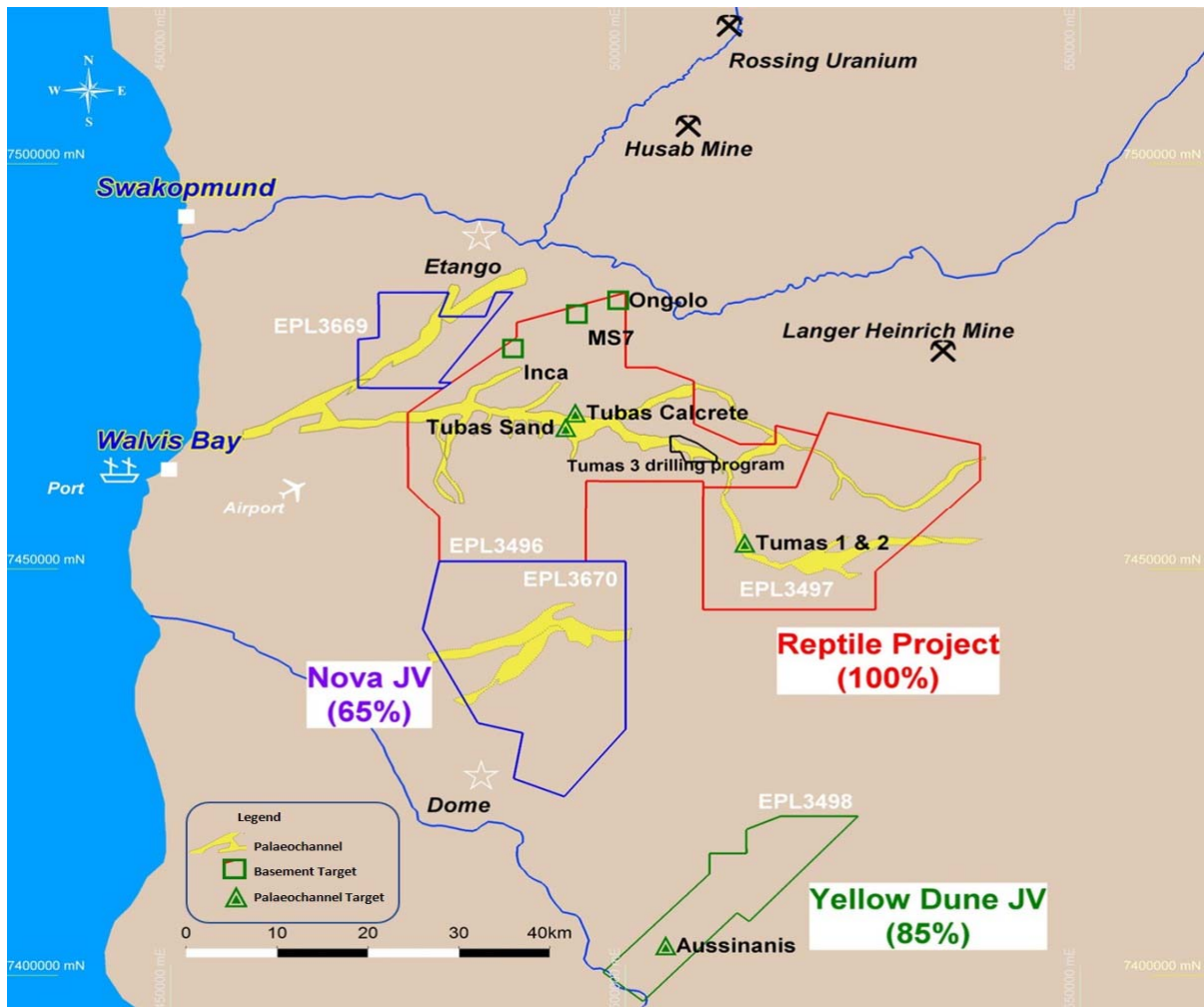
Figure 1: EPLs 3496, 3497 showing Tumas 3 and main prospect locations over prospective palaeochannels
