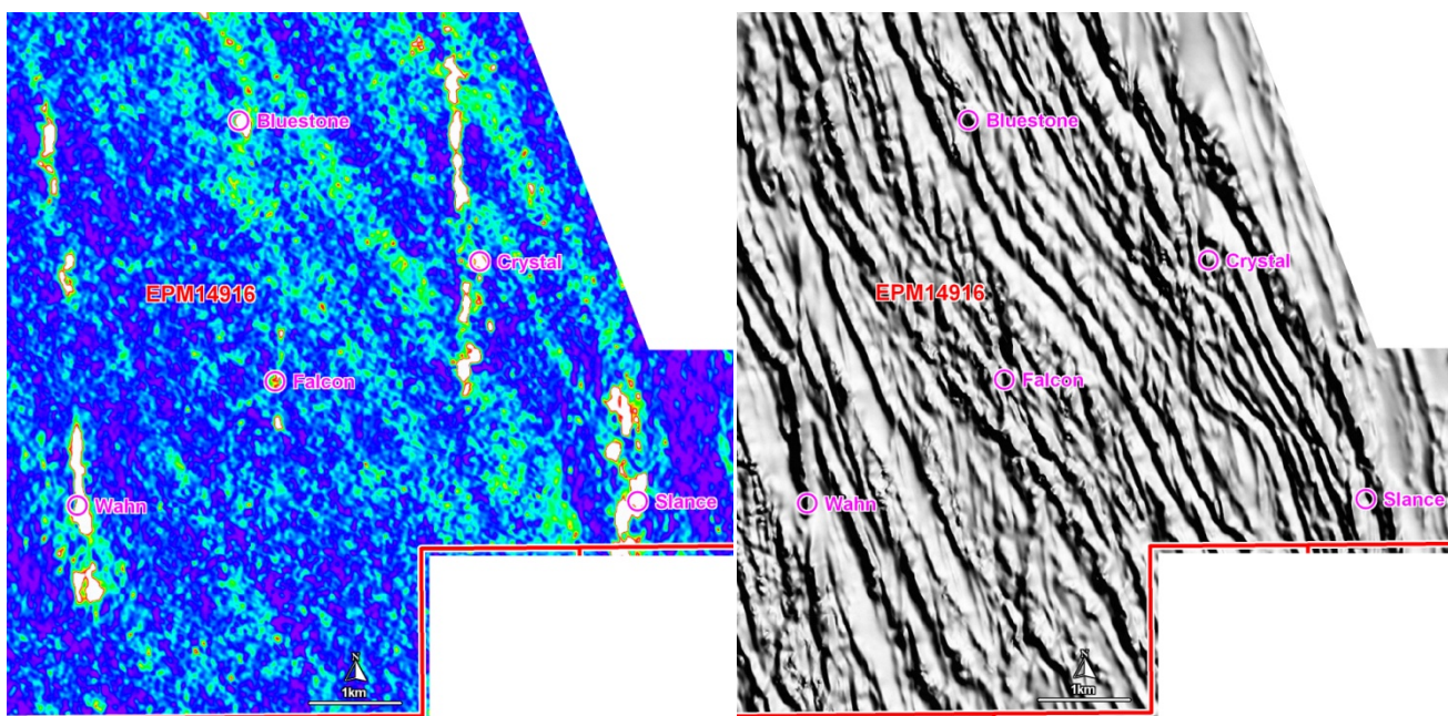
Figure 11: Airborne radiometric image with intense (white) uranium anomalies striking N-S. Right hand image 1VD magnetic showing NNW regional trend cut by later NS structures which host uranium mineralisation
